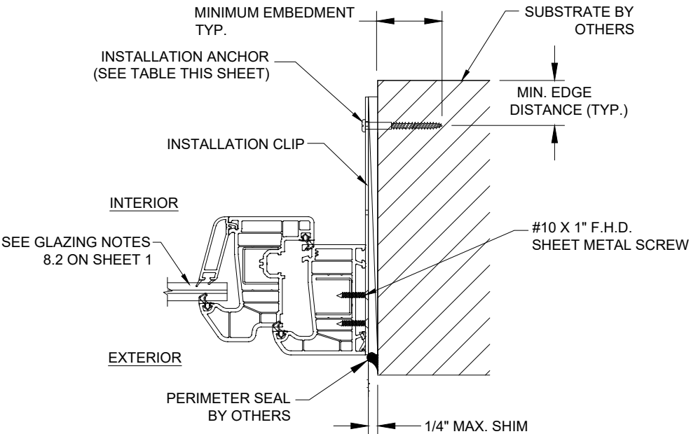
C 5 ANCHOR DETAIL INSTALLATION CLIP FRAME JAMB
