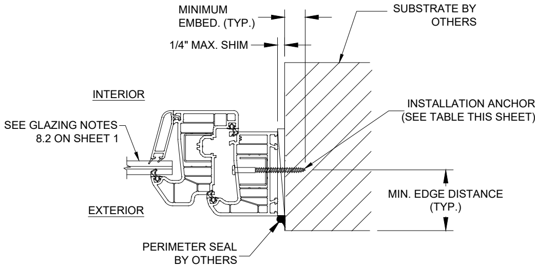
C 6 ANCHOR DETAIL THROUGH FRAME FRAME JAMB
