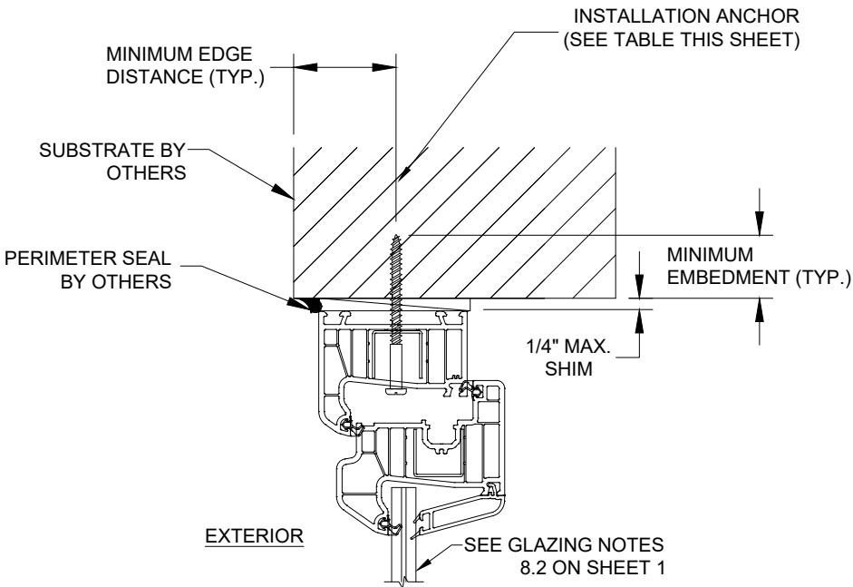
B 6 ANCHOR DETAIL THROUGH FRAME FRAME HEAD
